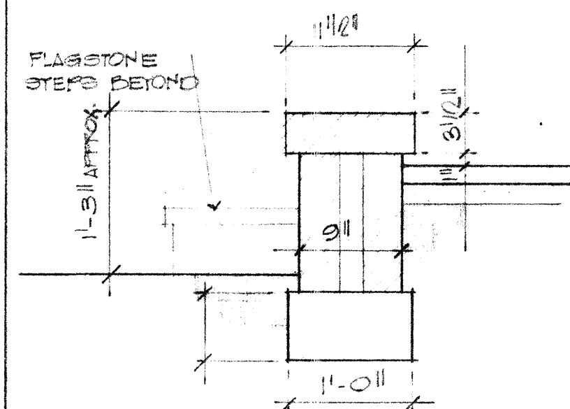
PATIO WALL 1'-0" 3.
