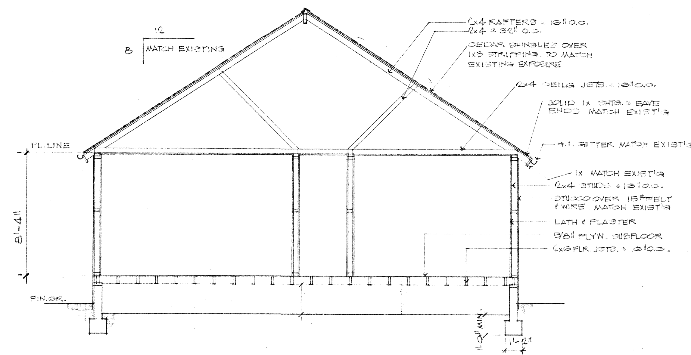
SECTION SCALE 1/4"=1'-0"
