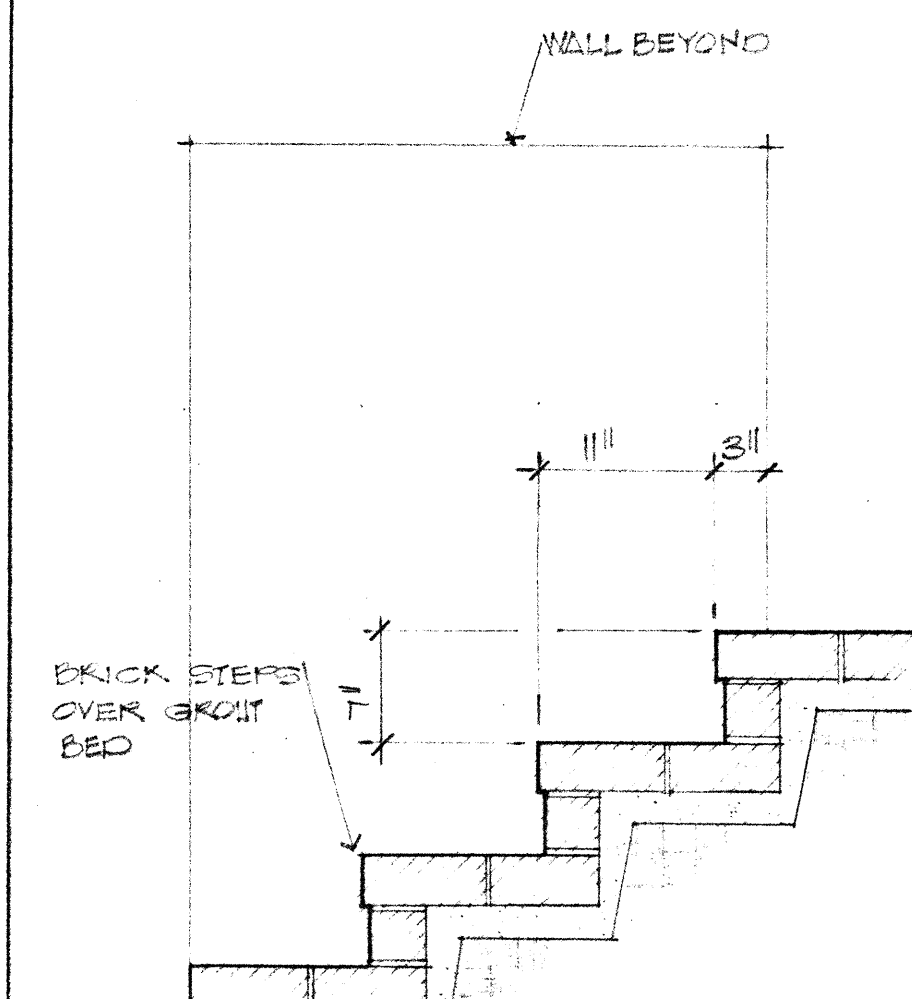
BRICK STEPS 1'-0" 2.
